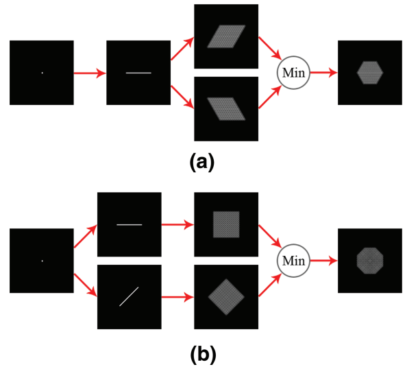
Figure 10: The filtering workflow for our separable hexagon (a) and octagon (b) implementations.
